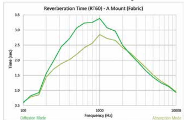
One 4' x 8' panel in reverberation room
